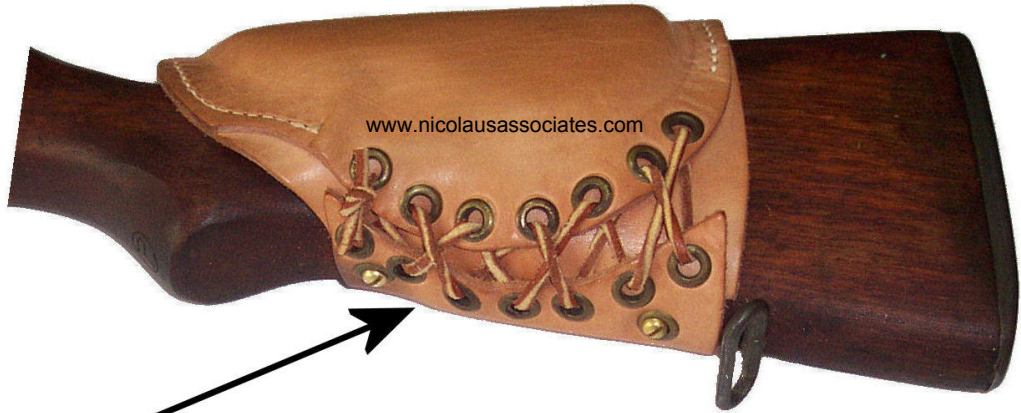
Cheek Pad Assembly - Installed on M1D Stock
